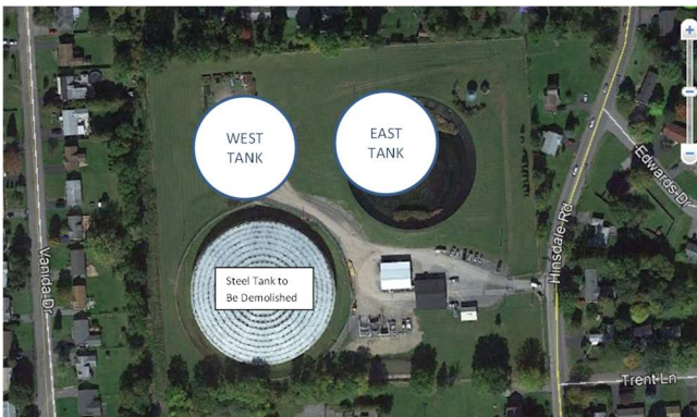
CONCEPTUAL LAYOUT OF FAIRMOUNT TANKS
